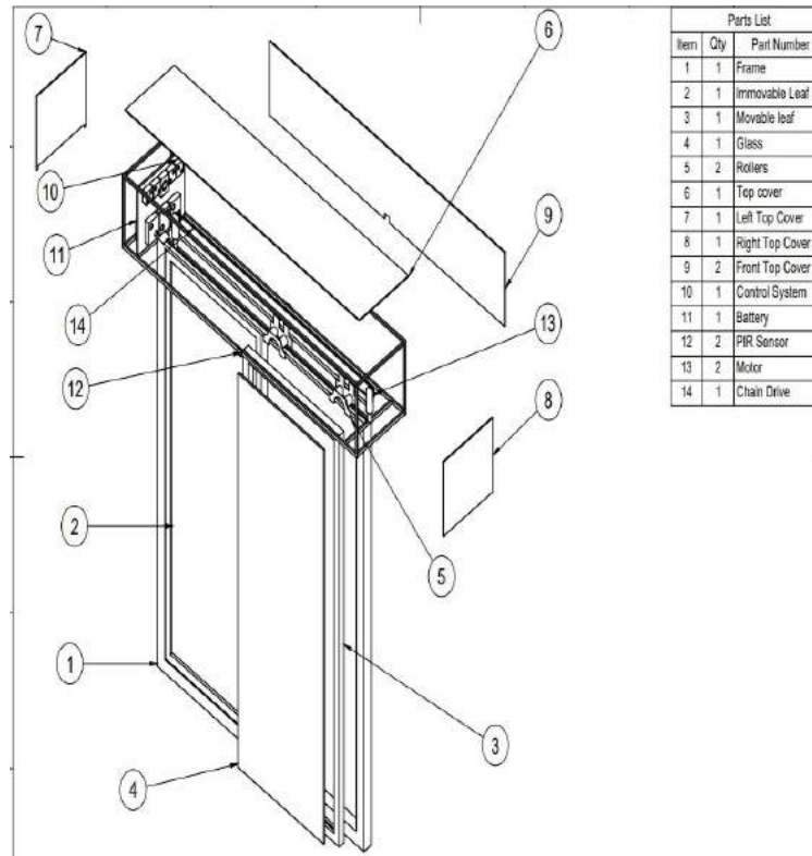
Figure 3 Exploded view of the self-opening and closing door
